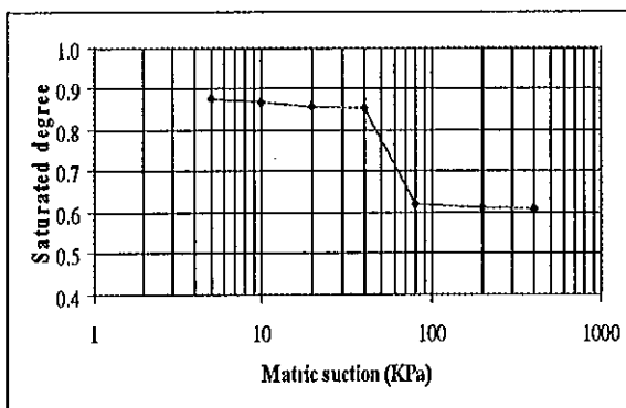
Fig. 1. Soil water characteristic curve of residual soils in Bac Kan ( dry curve ).
